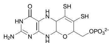
Fig. 1 Structure of molybdopterin 2
