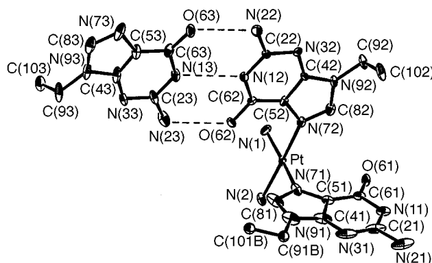
Fig. 10 Mismatch between \text{N}^7 platinated, \text{N}^1 deprotonated guanine and neutral guanine, as found in cis - [\text{Pt}(\text{NH}_3)_2(\text{egua})_2]\cdot\text{Hegua} (Hegua = 9-ethylguanine) 27
