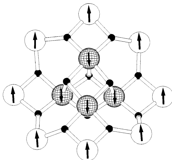
Fig. 7 Representation of the spin structure of the core of [\text{Mn}_{12}\text{O}_{12}(\text{O}_2\text{CCH}_3)_{16}(\text{H}_2\text{O})_4]^{20}
